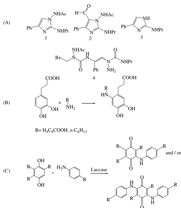
Figure 9 (A) N -[2-alkylamino-4-phenylimidazol-1-yl]-acetamide (substrate 1) and products 2-4 formed during incubation with T. versicolor laccase, (B) The natural compound 3-(3,4-dihydroxyphenyl)-propionic acid derivative can be synthesized by laccase-catalyzed N -coupling of aromatic and aliphatic amines, and (C) the coupling of p -hydroquinones with primary aromatic amines by laccases.
