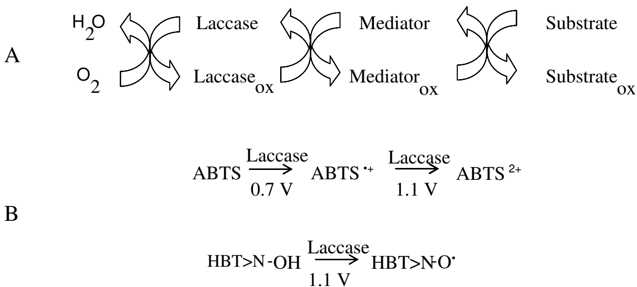
Figure 1 Expanded role of laccase oxidizing non-usual substrates by the action of redox mediators (A); and redox potentials of the oxidation reactions of ABTS and HBT by laccase (B).
