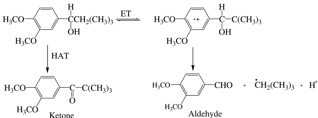
Figure 3 Diagram showing the differences between the oxidation mechanisms followed by ABTS radicals (Electron Transfer route, ET) and HBT radicals (Hydrogen Atom Transfer route, HAT) in LMS for oxidation of non-phenolic substrates (according to Galli and Gentili[52]).
