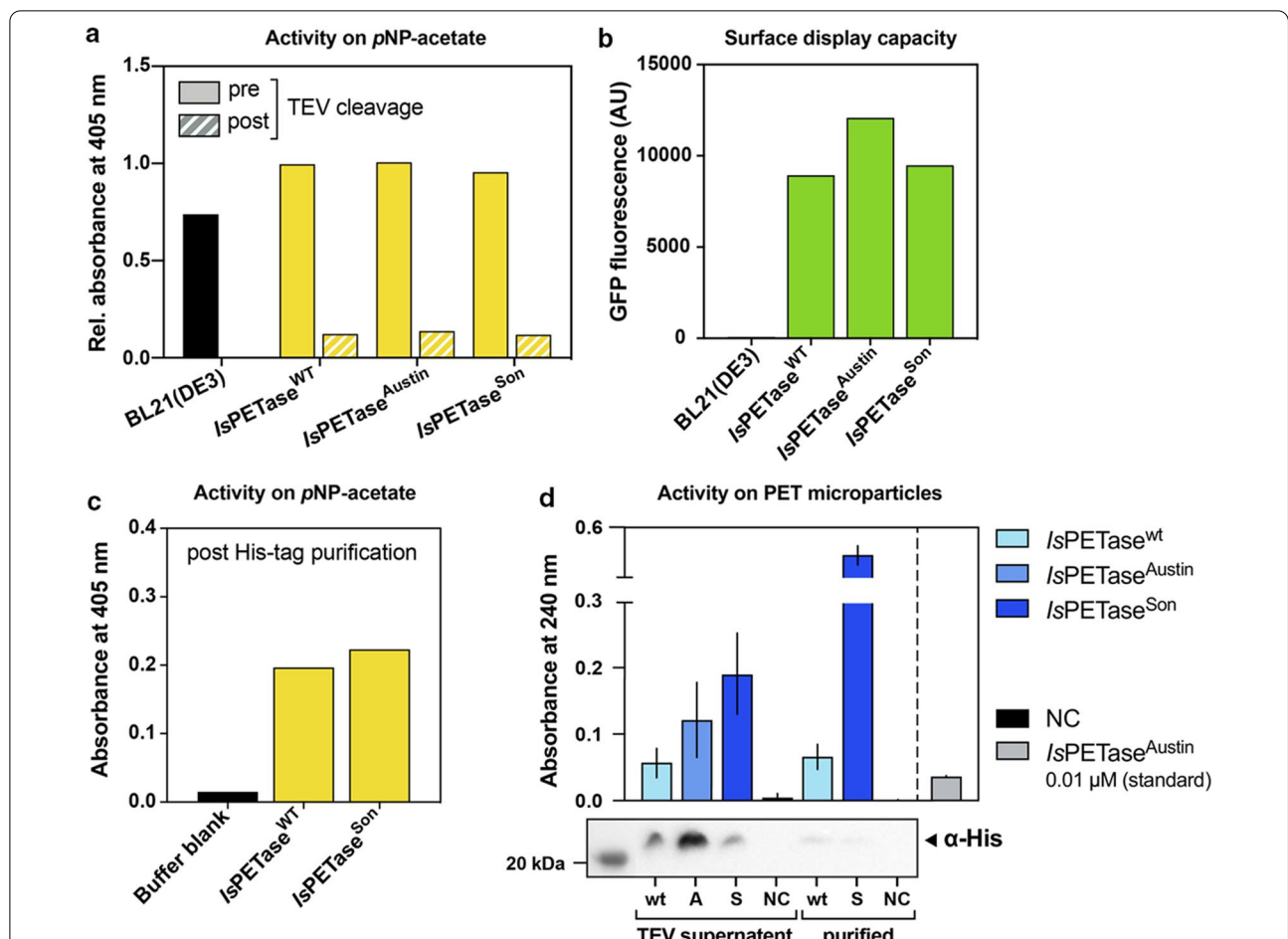
Fig. 4 Surface display and activity assessment of different IsPETase variants. a Activity of wt, Austin, and Son IsPETase variants expressed via the LppOmpA surface display module prior to and post TEV cleavage, hence release from the cell surface. To allow comparison of absorbance, values are relative to IsPETase WT activity prior to TEV cleavage. Expression of all samples was performed at 16 °C. b Whole-cell fluorescence verification of surface-displayed IsPETase variants (wt, Austin, Son) prior to TEV cleavage. c Activity of IsPETase WT and IsPETase Son on pNP-acetate after His-tag purification. Buffer blank: 50 mM HEPES buffer. d Activity and detection of the previously described IsPETase variants expressed on the surface and subsequently cleaved off (TEV supernatant) and His-tag purified (purified). Activity of the released IsPETase variants on PET microparticles (upper half) and detection of the His-tagged enzymes via western blot (lower half) using an anti-His antibody. NC: Negative control BL21(DE3) cells
